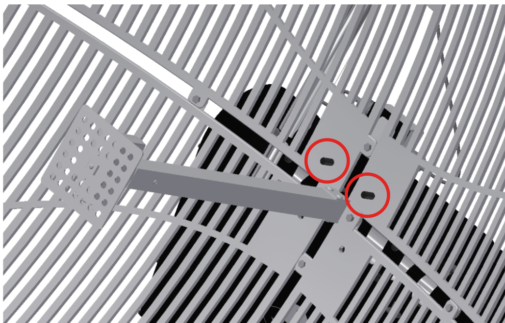
Fitting antenna
